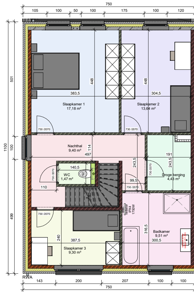
Verdieping LL - lot 11
