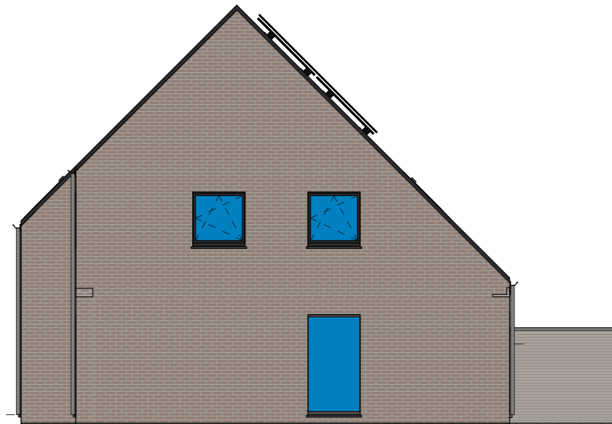
LL Rechtergevel lot 170
