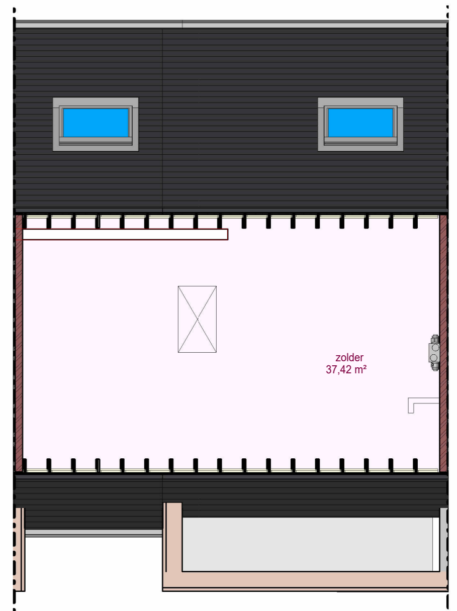
3 Zolder verdieping 184 LL 1 : 70
