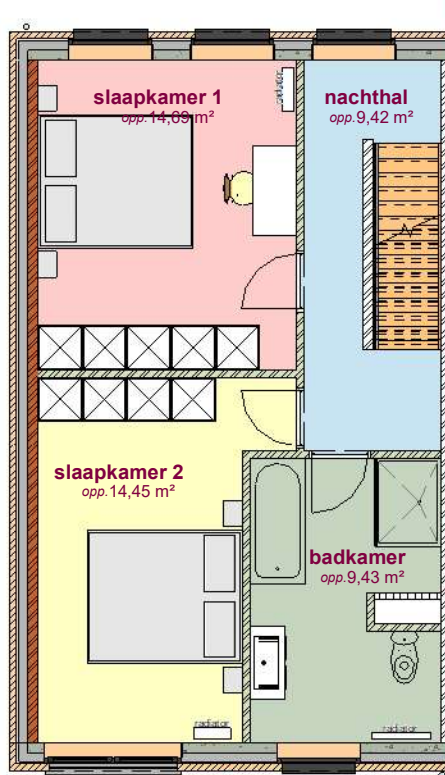
Lot 11 verdieping - lot 11 LL
