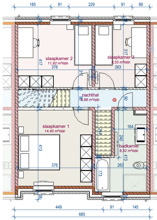
lot B6 verdieping
